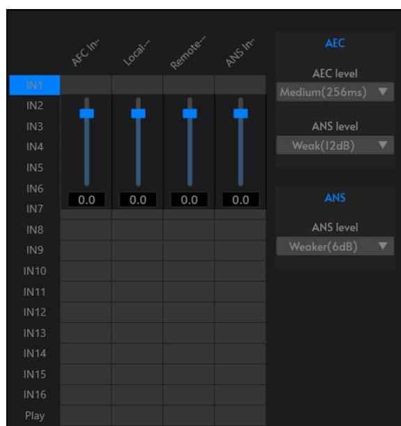
Example, AFC and Matrix Mixer association operations
